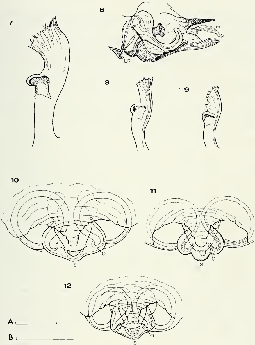
FIGS 6–12. - 6, Centromerus bulgarianus (Drensky), suprategulum and embolic division (Suhata Pestera Cave, Bulgaria); 7, C. dacicus Dumitrescu & Georgescu, terminal apophysis (Closani Cave, Romania) (DUMITRESCU & GEORGESCU 1980); 8, C. prope dacicus Dumitrescu & Georgescu, terminal apophysis (Zlotska Pečina Cave, Serbia); 9, C. bulgarianus (Drensky), terminal apophysis (Suchata peatera Cave, Bulgaria); 10, C. prope dacicus Dumitrescu & Georgescu, vulva and epigyne (Zlotska Pečina Cave, Serbia); 11, C. dacicus Dumitrescu & Georgescu, vulva and epigyne (Closani Cave, Romania) (DUMITRESCU & GEORGESCU 1980); 12, C. bulgarianus (Drensky), vulva and epigyne (Suchata Pestera, Bulgaria). Scale line 0.10 mm (6, 8, 9, 10, 12). Figs 7, 11 is taken from DUMITRESCU & GEORGESCU 1980 (no scale line).
